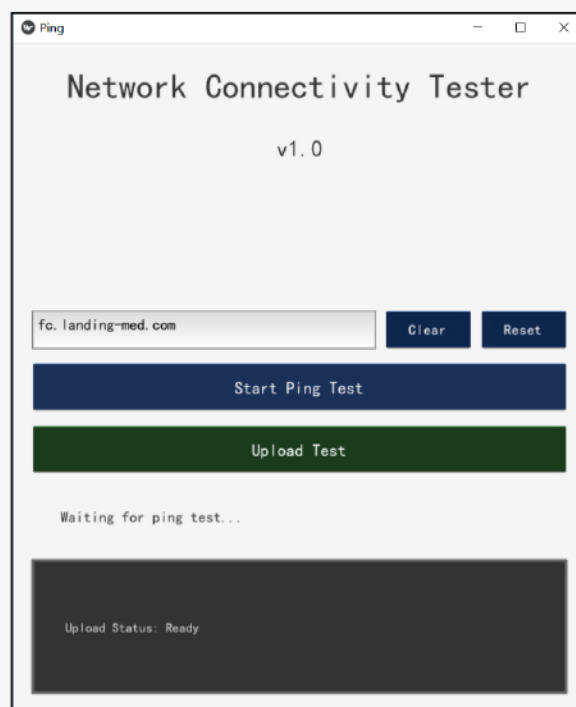
Figure 2 Software Interface
